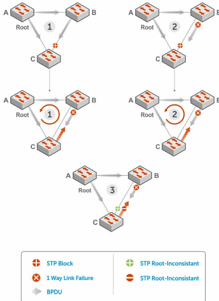
Figure 115. STP Loop Guard Prevents Forwarding Loops
